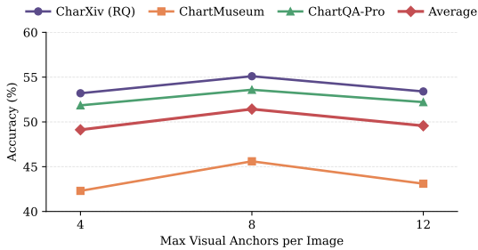
Figure 6: Performance under different maximum numbers of visual anchors per image.
