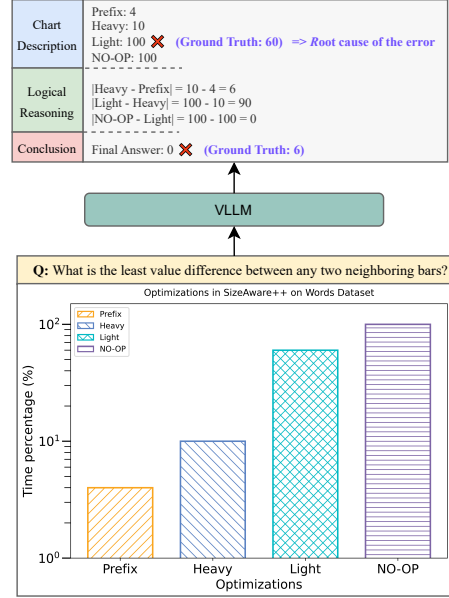
Figure 1: Given a bar chart and a reasoning question, a VLLM first generates a description of each bar, and then compares each pair of values to give the final answer. The error stems from the initial visual perception.
