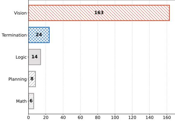
Figure 2: Statistics of failure cases in chart reasoning. As a sample may have multiple errors, total labels (215) exceed samples (200).
