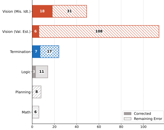
Figure 5: Breakdown of samples corrected by Chart-EARL vs. remaining errors within 200 sampled errors in the pilot experiment.
