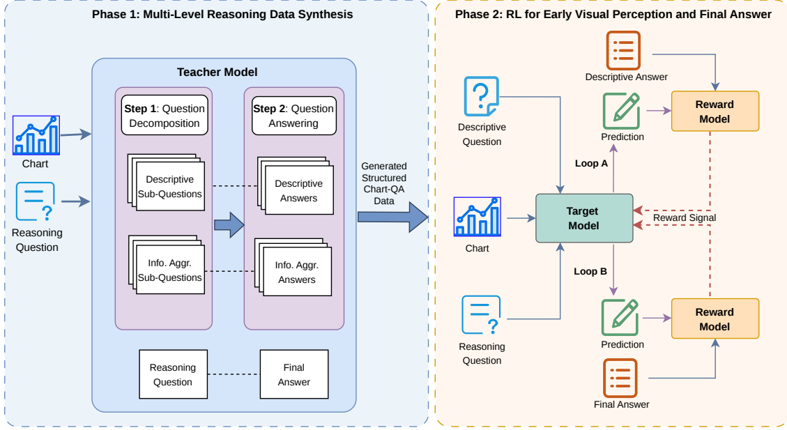
Figure 3: Overview of Chart-EARL . Phase 1 synthesizes structured data by decomposing queries into vision perception, information aggregation, and final reasoning. Phase 2 utilizes a dual-objective RL framework, combining our proposed early visual anchoring (Loop A) with standard outcome supervision (Loop B).
