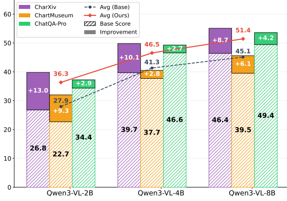
Figure 4: Performance breakdown across different model scales (2B, 4B, 8B). The stacked bars represent accuracy on benchmarks (color-coded). The hatched lower portion represents the baseline performance, while the solid upper portion denotes the absolute performance gain contributed by Chart-EARL. The overlaid lines depict the average accuracy trend, contrasting the baseline (dashed line) with our method (solid red line).
